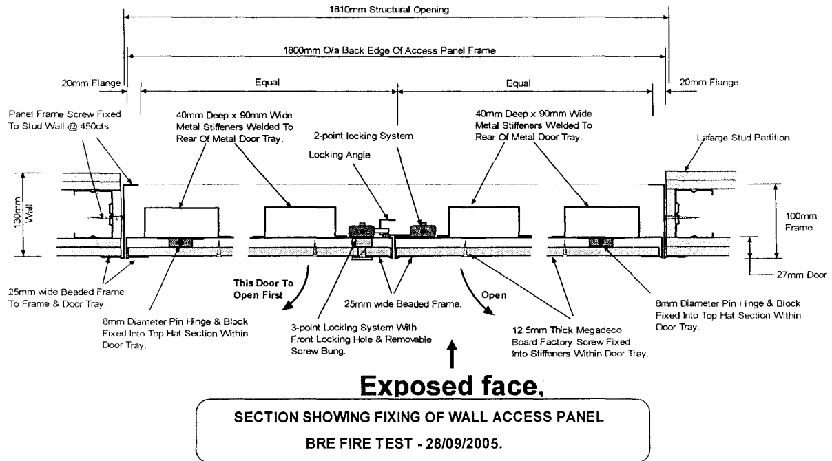
Figure 2 Showing a horizontal section through the access panel. (view is from below)
